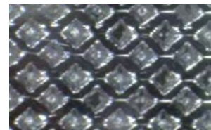
Anilox roll after Special Blade Clean wash
